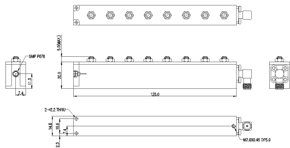
X-Band TX CH Filter
