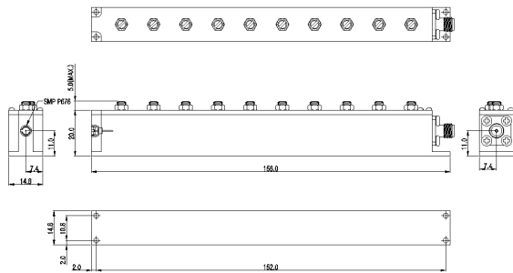
X-Band RX CH Filter
